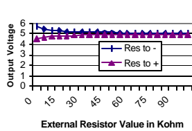
PM3012S05 Voltage Trim Adjust
