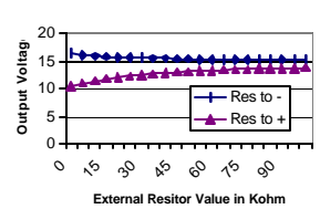
PM3012S15 Voltage Trim Adjust
