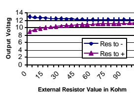
PM3012S12 Voltage Trim Adjust
