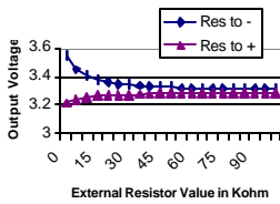
PM3012S03 Voltage Trim Adjust
