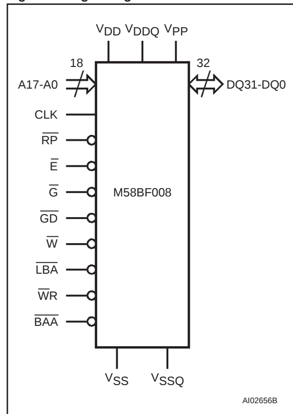
Figure 2. Logic Diagram
