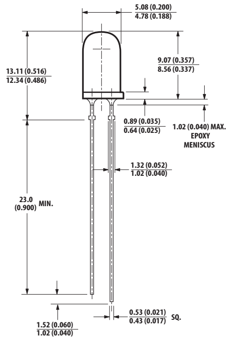
PACKAGE OUTLINE "C" HLMP-1340/1440/1540
