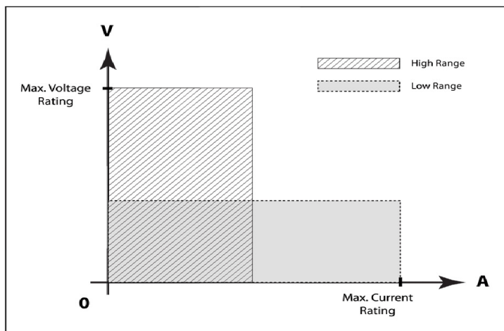
9170/9180 Series Operating Range
