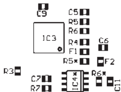
Fig. 4.4.: Bottom side USB Infrared-Transceiver
