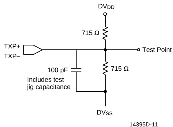
TXP Switching Test Circuit
