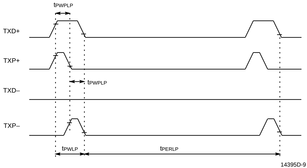
TP Idle Link Test Pulse
