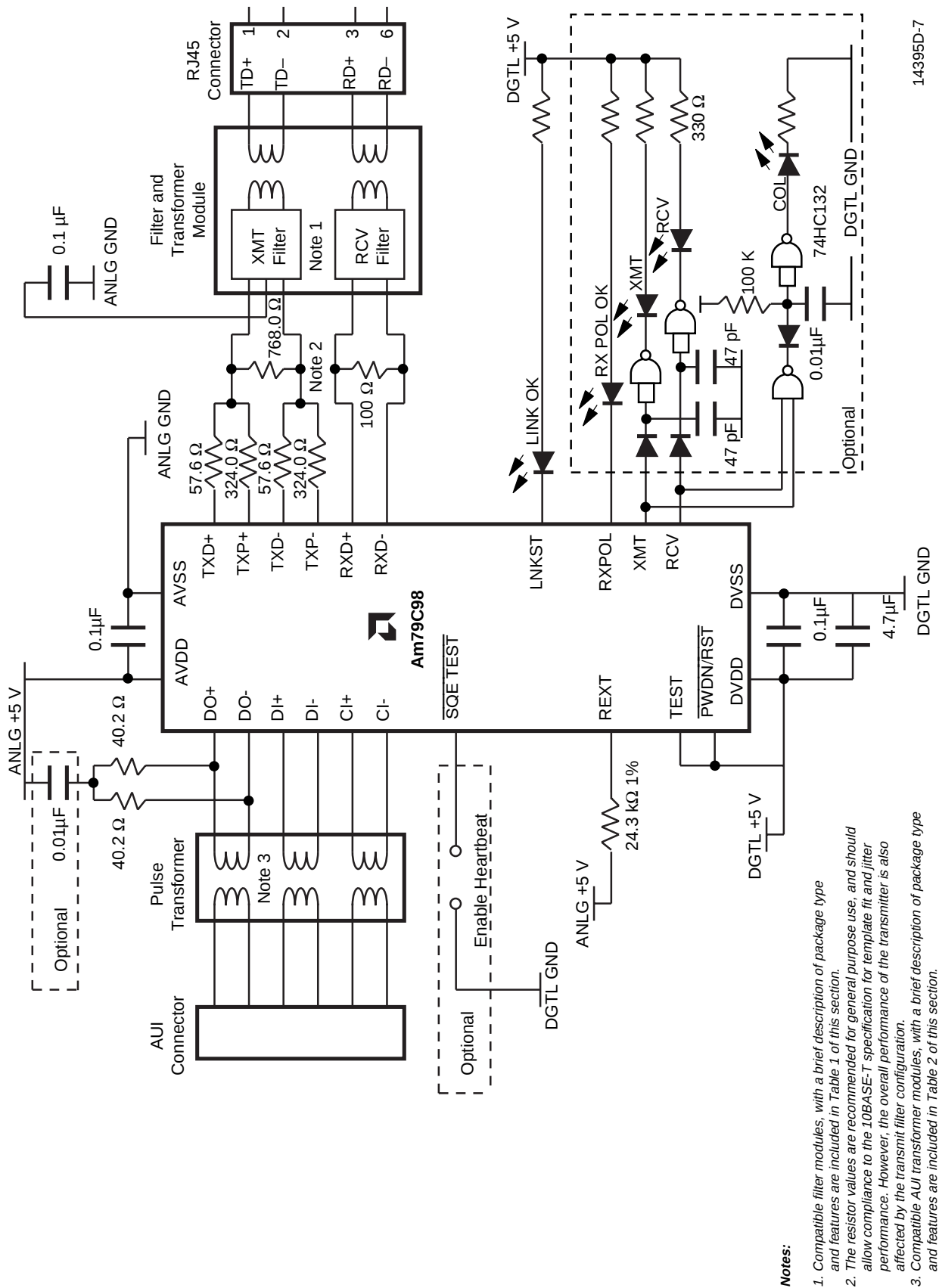
Figure 3. Typical TPEX System Application
