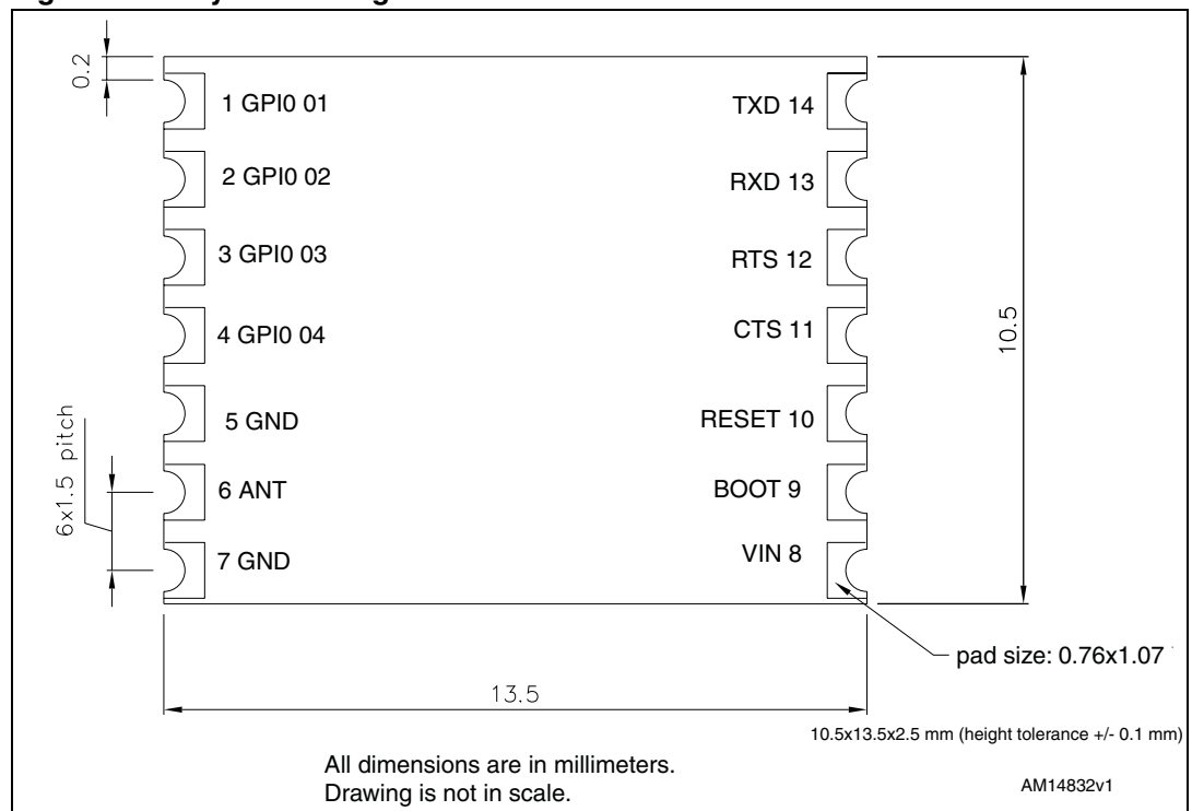
Figure 4. Layout drawing
