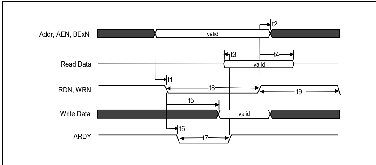
FIGURE 7-1: ASYNCHRONOUS CYCLE
