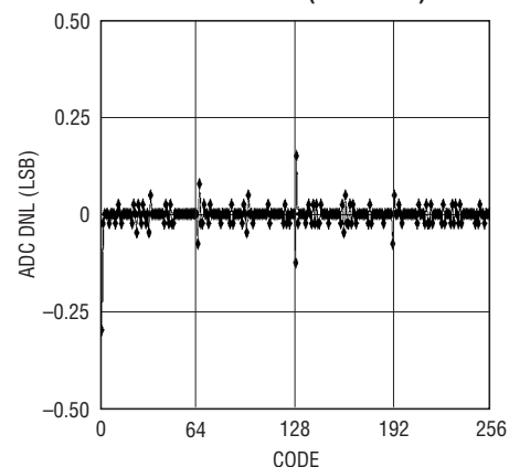
ADC DNL vs Code (ADIN Pin)
