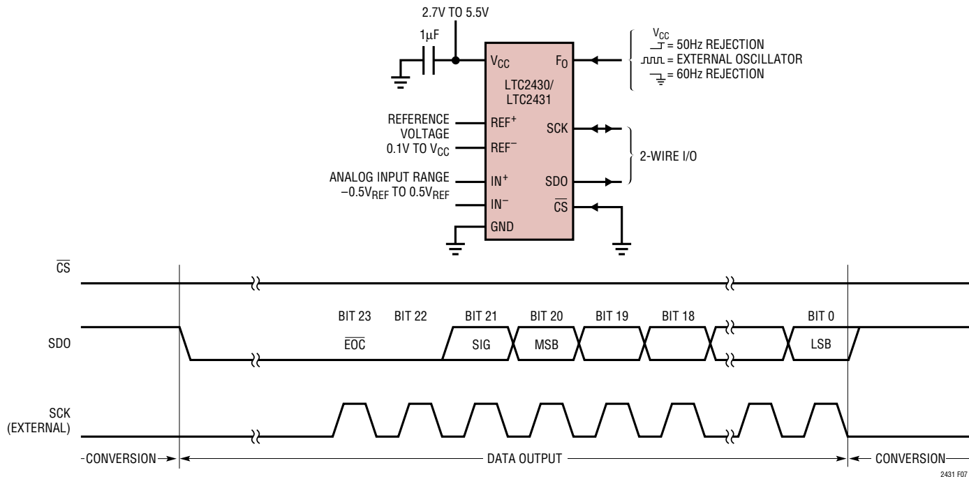
Figure 7. External Serial Clock, \overline{\text{CS}} = 0 Operation
