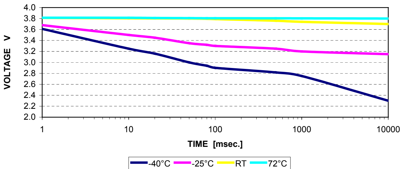
VOLTAGE vs. TIME CURVES for HLC-1520A at Li/SO 2 Cl 2 potential, 350 mA.
