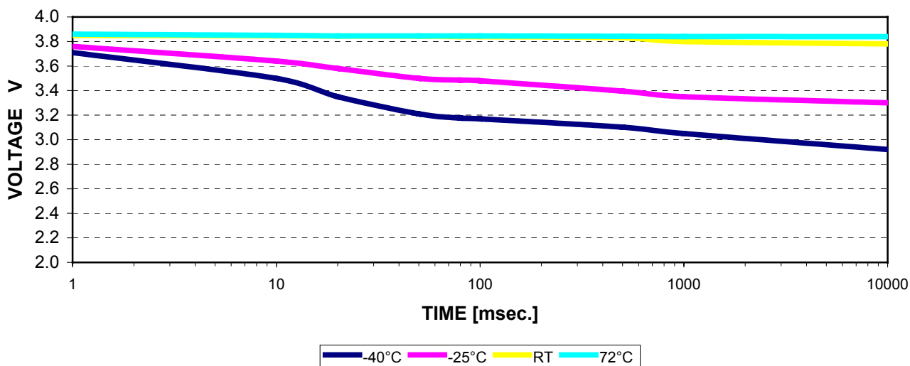
VOLTAGE vs. TIME CURVES for HLC-1520A at Li/SO 2 Cl 2 potential, 200 mA.
