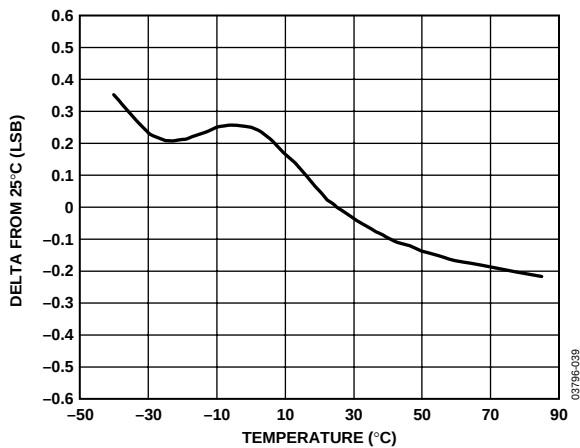
Figure 7. Change in ADC Gain vs. Temperature
