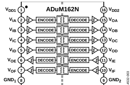
Figure 3. ADuM162N Functional Block Diagram
