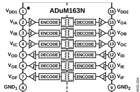
Figure 4. ADuM163N Functional Block Diagram
