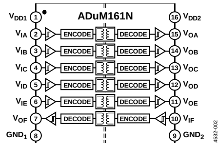
Figure 2. ADuM161N Functional Block Diagram
