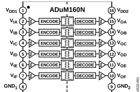
Figure 1. ADuM160N Functional Block Diagram
