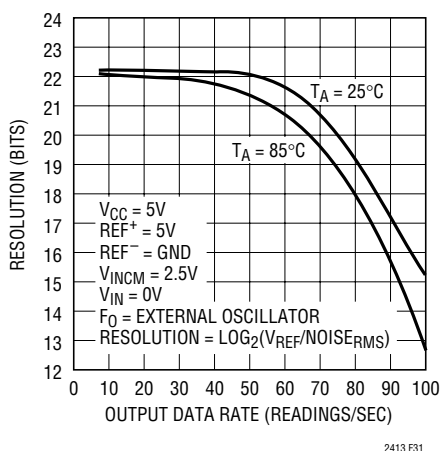
Figure 31. Resolution ( \text{Noise}_{\text{RMS}} \leq 1\text{LSB} ) vs Output Data Rate and Temperature
