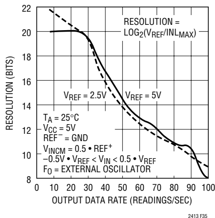
Figure 35. Resolution ( \text{INL}_{\text{MAX}} \leq 1\text{LSB} ) vs Output Data Rate and Reference Voltage
