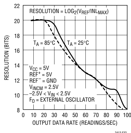
Figure 32. Resolution ( \text{INL}_{\text{RMS}} \leq 1\text{LSB} ) vs Output Data Rate and Temperature
