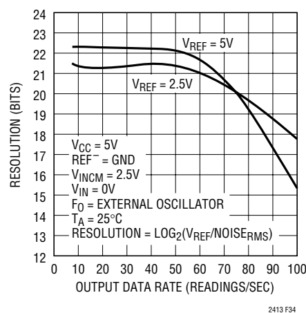
Figure 34. Resolution ( \text{Noise}_{\text{RMS}} \leq 1\text{LSB} ) vs Output Data Rate and Reference Voltage
