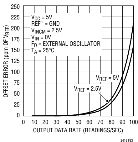
Figure 33. Offset Error vs Output Data Rate and Reference Voltage
