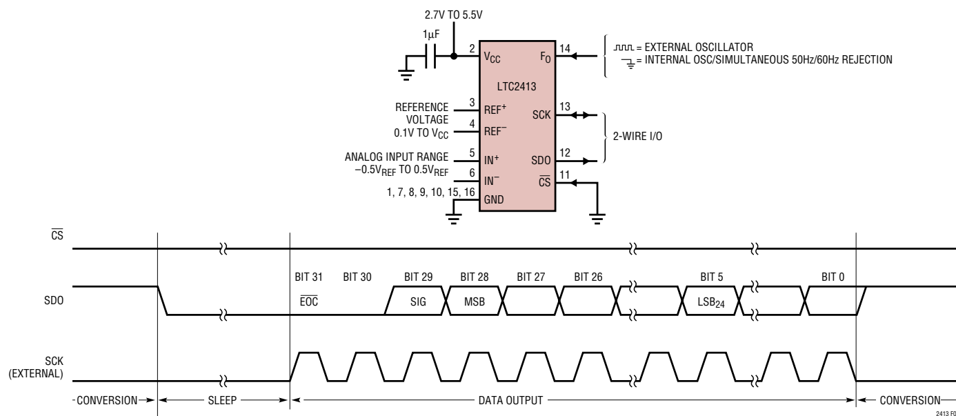
Figure 8. External Serial Clock, \overline{CS} = 0 Operation
