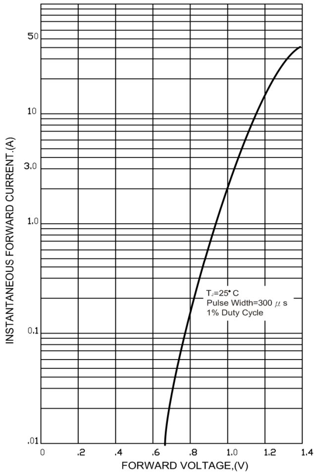
FIG.3-TYPICAL FORWARD CHARACTERISTICS
