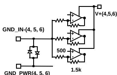
CIRCUIT 5
