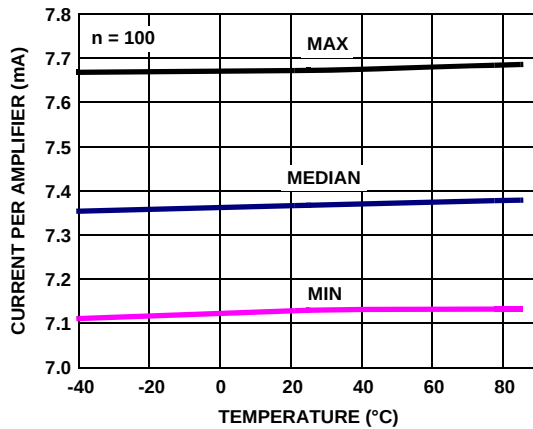
FIGURE 21. ENABLED SUPPLY CURRENT vs TEMPERATURE, V_S = \pm 2.5V
