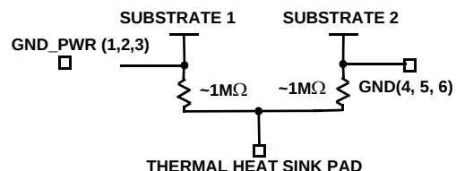
CIRCUIT 6
