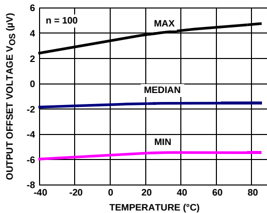
FIGURE 23. OUTPUT OFFSET VOLTAGE V_{OS} vs TEMPERATURE, V_S = \pm 2.5V , R_L = 1k
