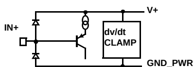
CIRCUIT 1
