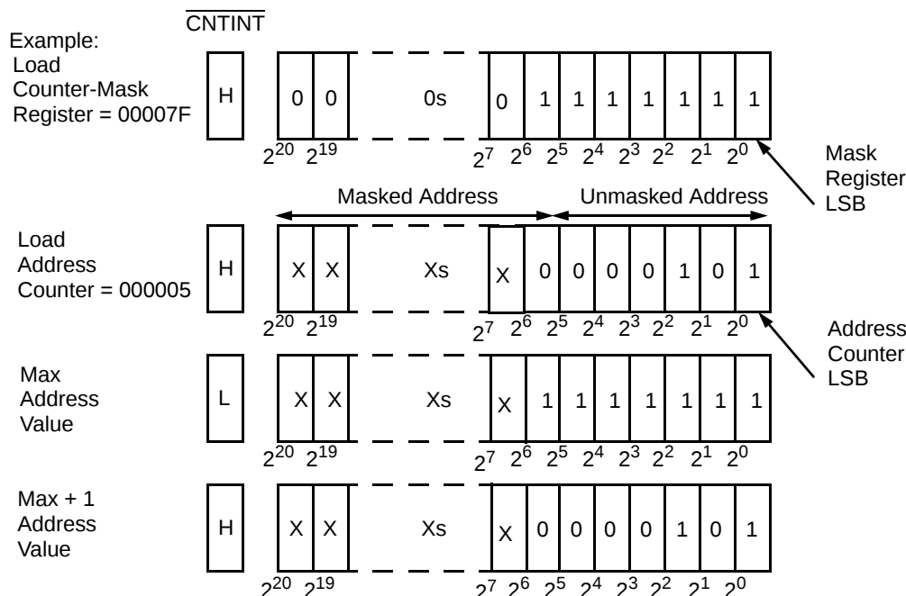
Figure 8. Programmable Counter-Mask Register Operation with \overline{\text{WRP}} deasserted
