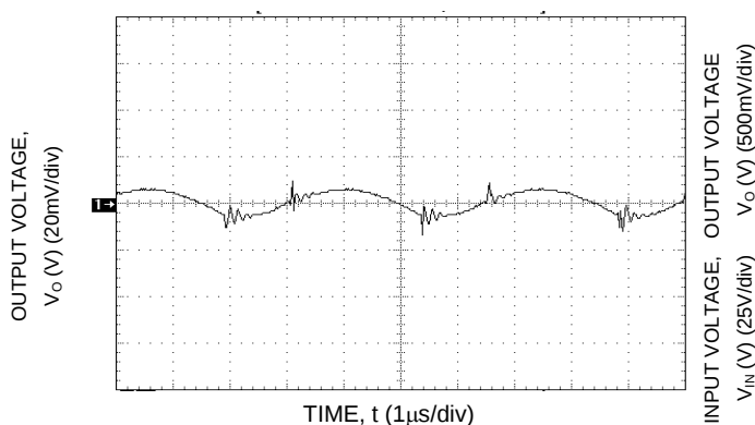
Figure 32. Typical Output Ripple and Noise.
