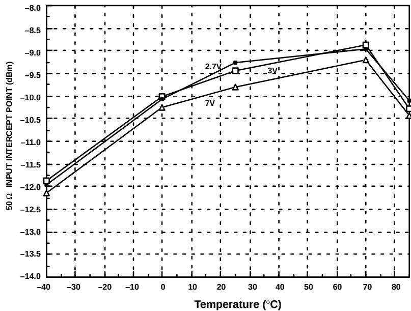
Figure 5. Third Order Intercept Point vs Supply Voltage
