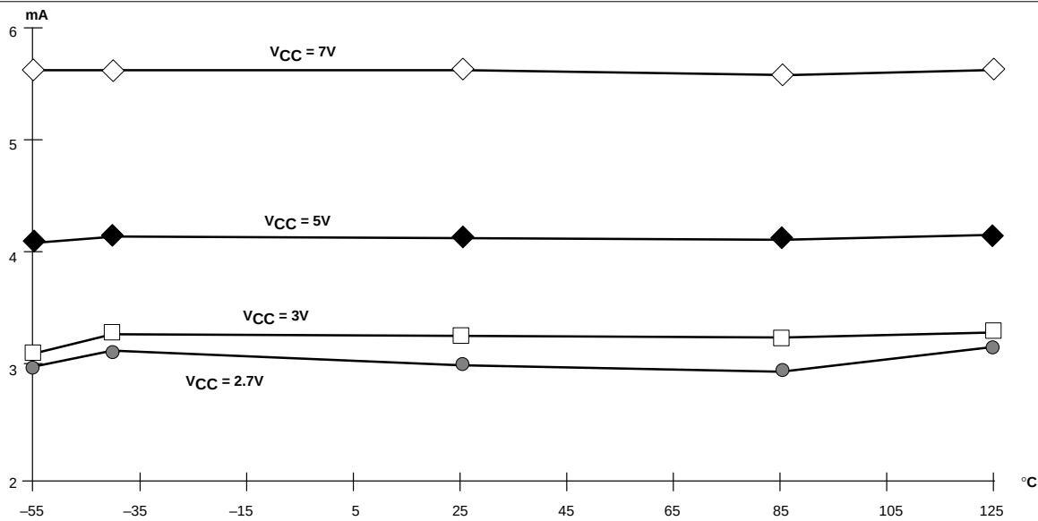
Figure 4. I_{CC} vs Temperature
