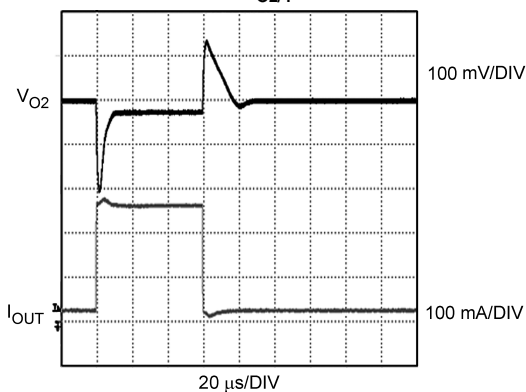
Load Transient Response V_{O2/4}
