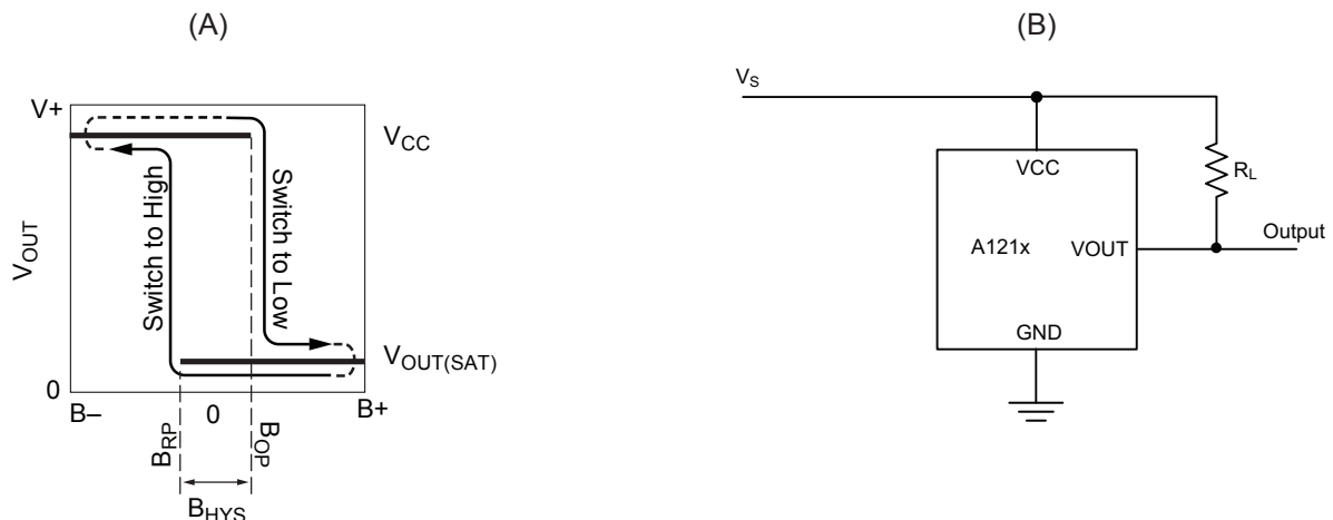
Figure 1: Switching Behavior of Latches
