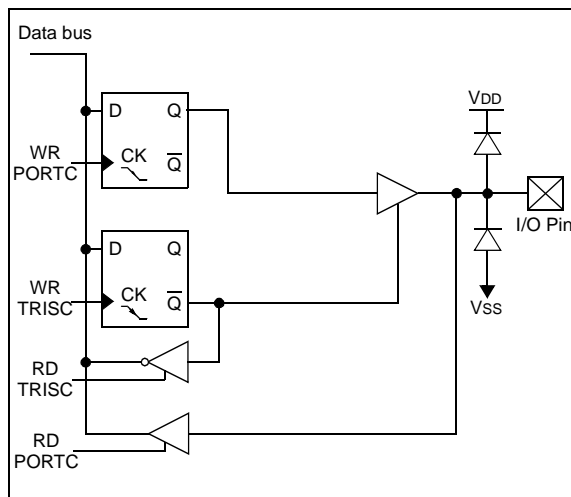
FIGURE 3-7: BLOCK DIAGRAM OF RC4 AND RC5 PINS
