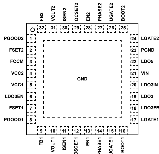
ISL62381, ISL62382, ISL62381C, ISL62382C (32 LD TQFN) TOP VIEW
