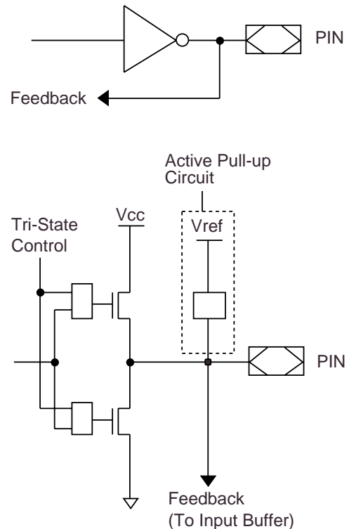
Typical Output
