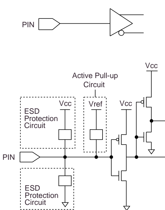
Typical Input
