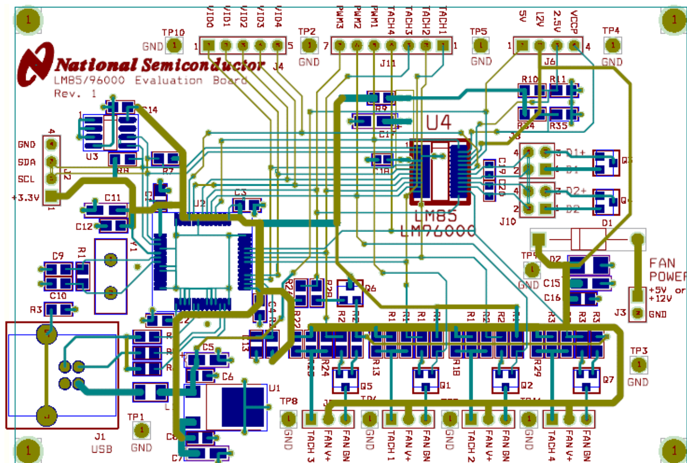
Figure 5.3 Layout diagram of the LM85/LM96000 Evaluation Board
