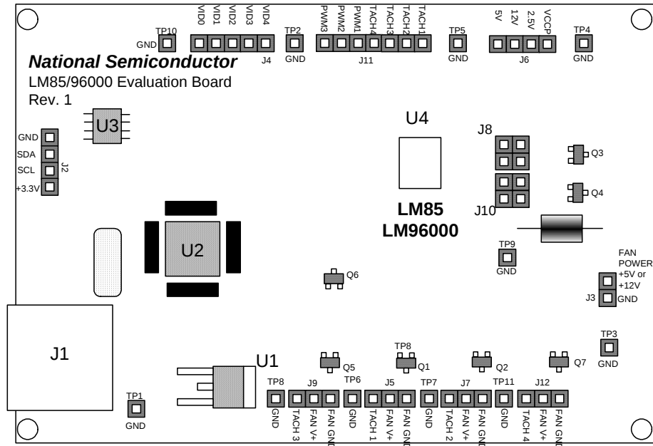
Figure 2.1.1 Physical Layout of the LM85/LM96000 Evaluation Board
