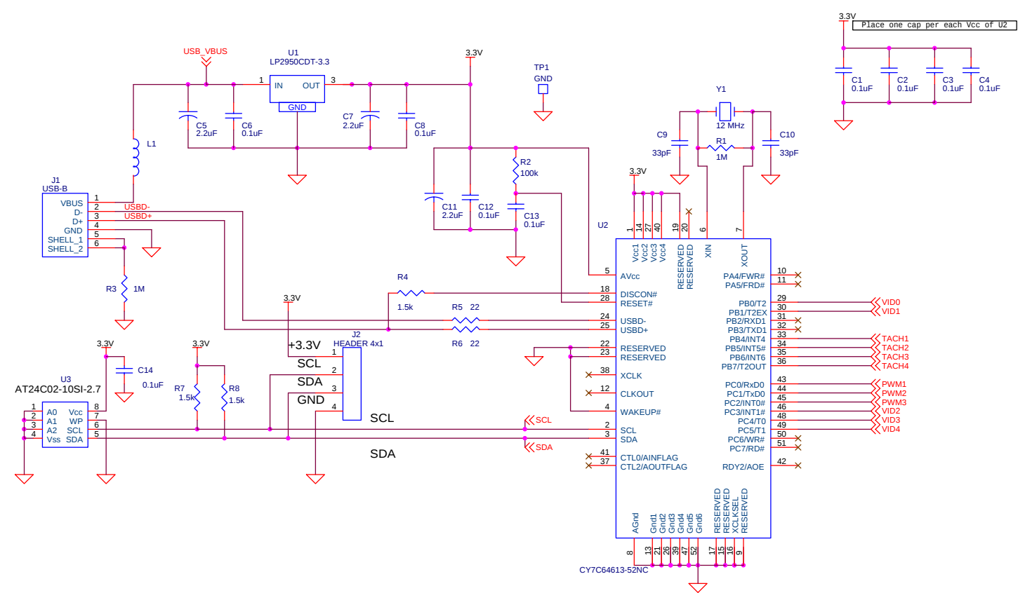
Page 1 of 2 Pages of the Schematic of the LM85/LM96000 Evaluation Board
