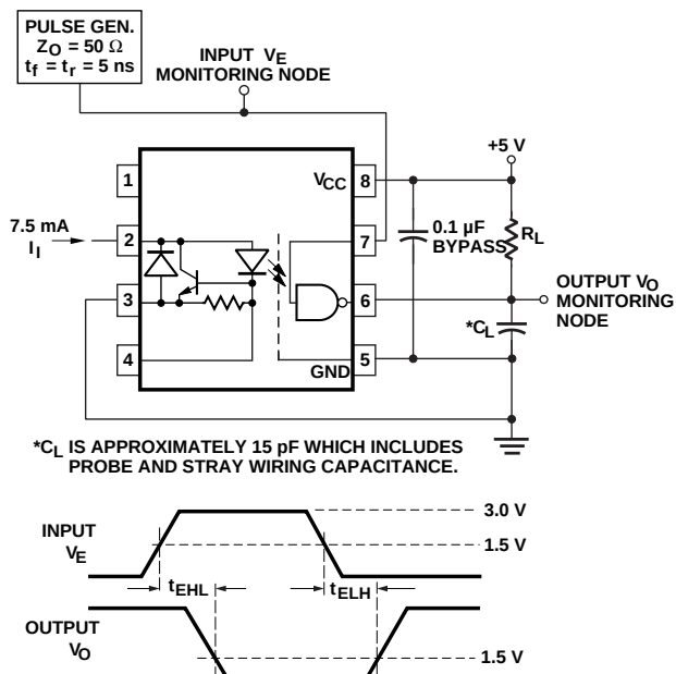
Figure 10. Test circuit for t eHL and t eHL *
