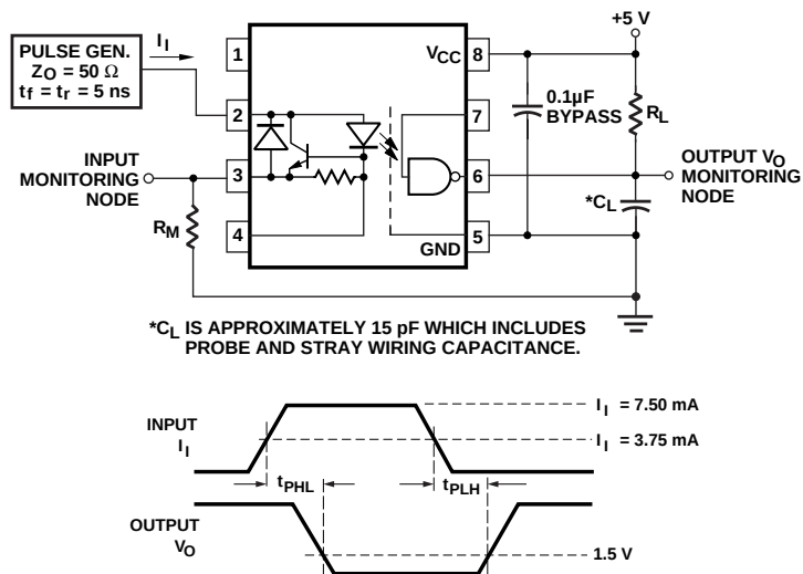
Figure 6. Test circuit for t pLH and t pLH *
