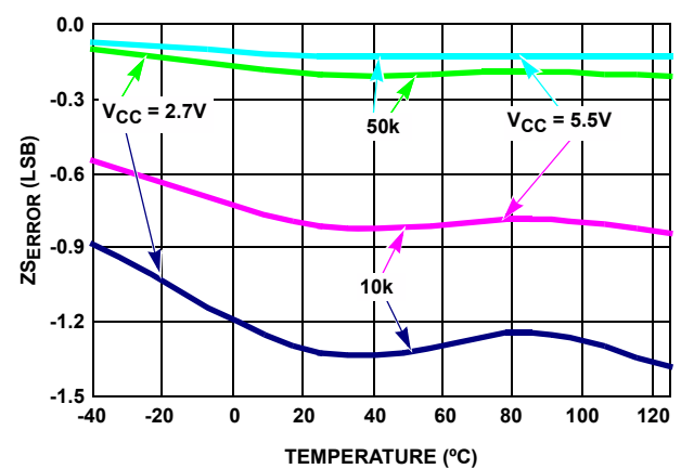
FIGURE 6. ZSERROR vs TEMPERATURE
