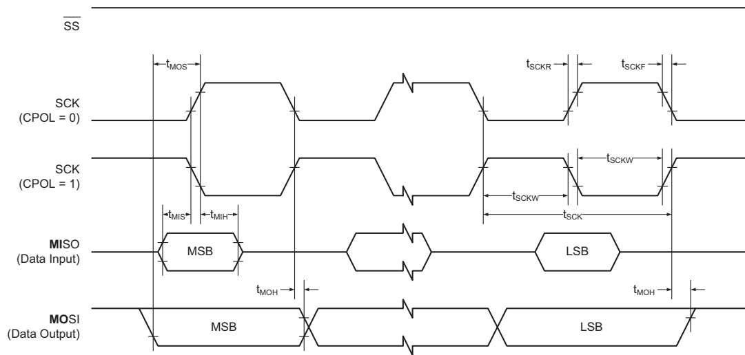
Figure 33-19. SPI timing requirements in master mode.
