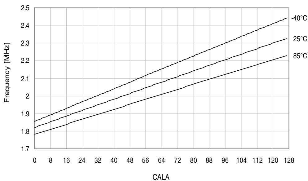
Figure 34-328. 2MHz internal oscillator frequency vs. CALA calibration value. V_{CC} = 3V .
