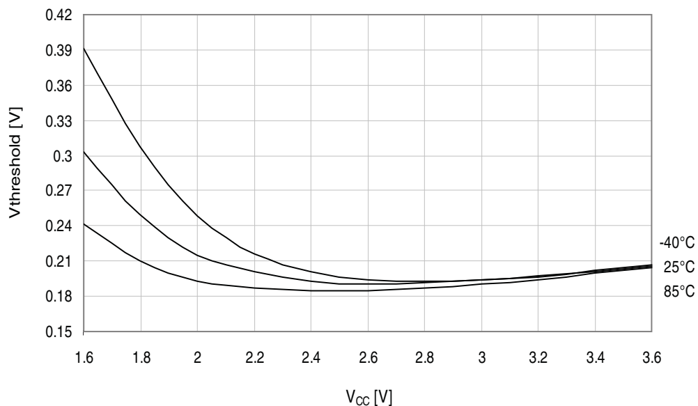
Figure 34-232. I/O pin input hysteresis vs. V_{CC} .
