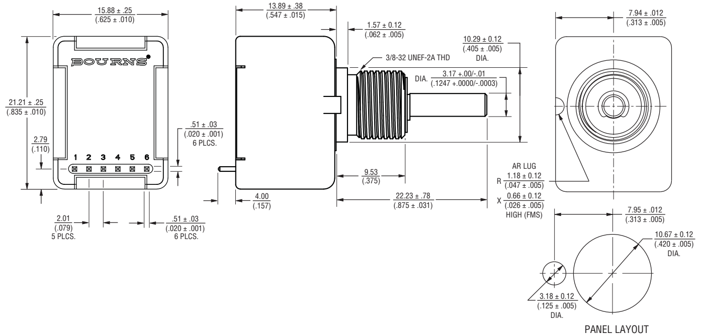
PANEL LAYOUT
