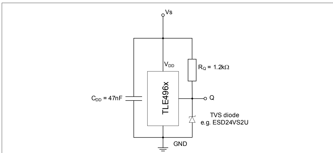
Figure 3-2 Enhanced Application Circuit #2 for extended ESD robustness
