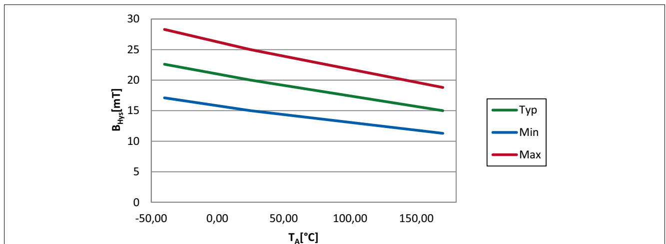
Figure 5-3 Hysteresis ( B_{Hys} ) of the TLE4961-4M over Temperature
