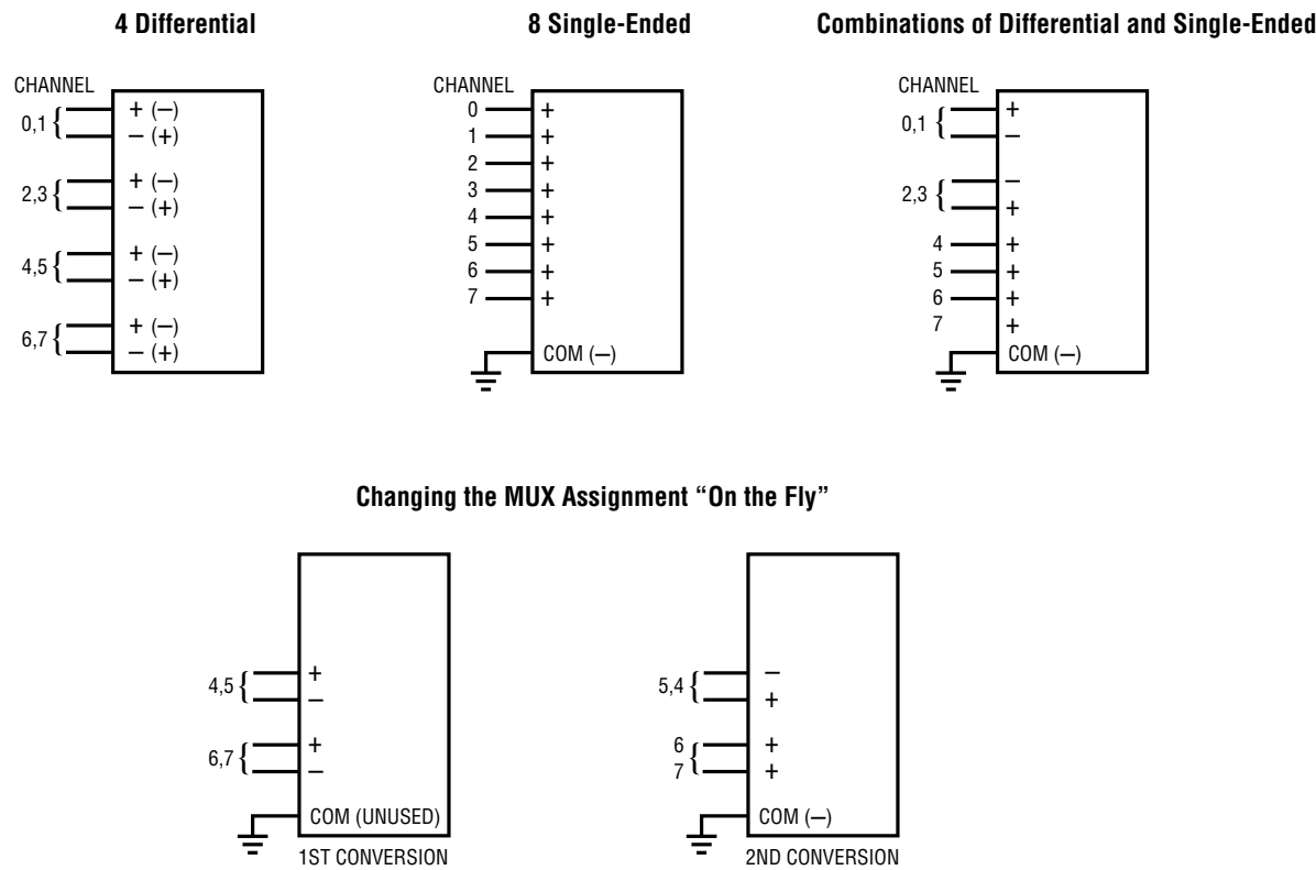
Figure 1. Examples of Multiplexer Options on the LTC1289
