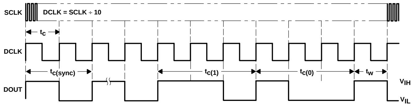
Figure 1. Timing Diagram
