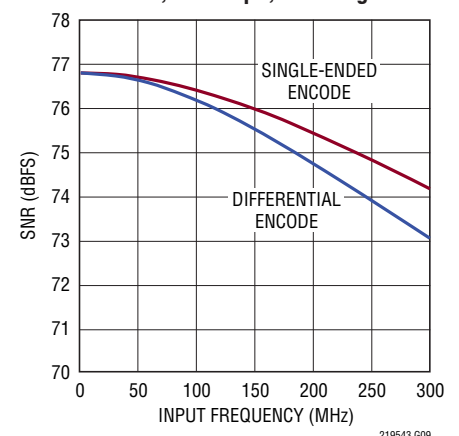
LTC2195: SNR vs Input Frequency, -1\text{dBFS} , 125\text{Mps} , 2\text{V} Range
