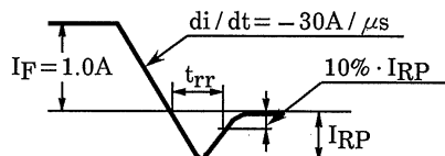
WAVEFORM
