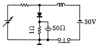
Note 1: t_{rr} TEST CIRCUIT
