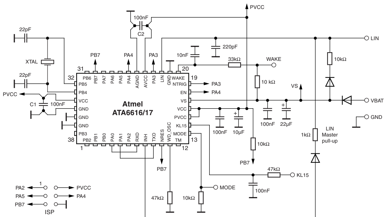
Figure 5-4. Typical LIN Master Application 1k \Omega LIN Master Pull-up Switched Off during Sleep and Silent Mode
