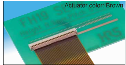
FH19SC – FPC/FFC thickness: 0.3 \pm 0.03\text{mm}
