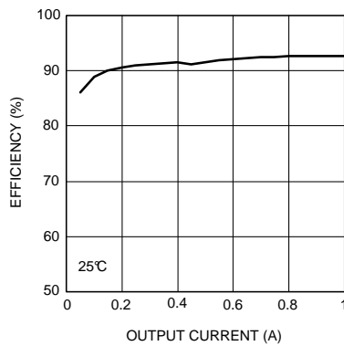
Figure 37. Efficiency
