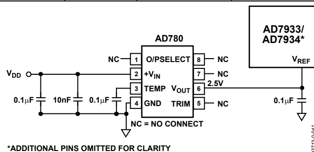
Figure 36. Typical V_{REF} Connection Program
