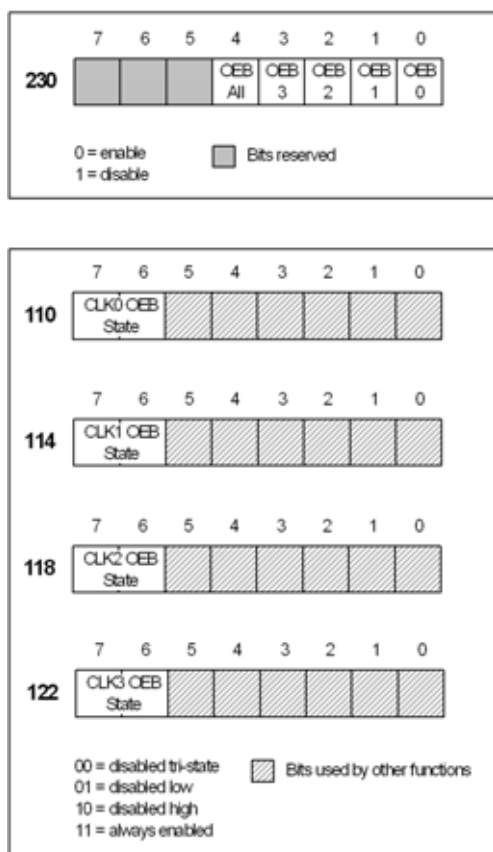
Figure 13. Output Enable Control Registers
