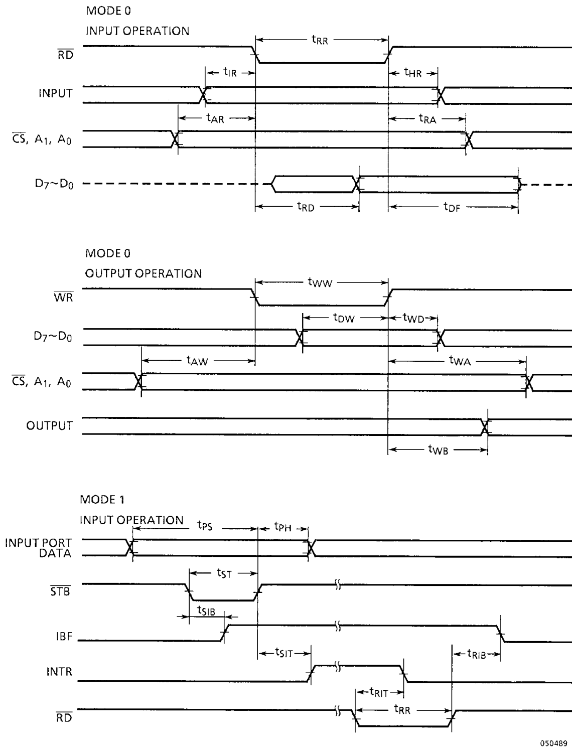
Figure 7.1 Timing diagram
