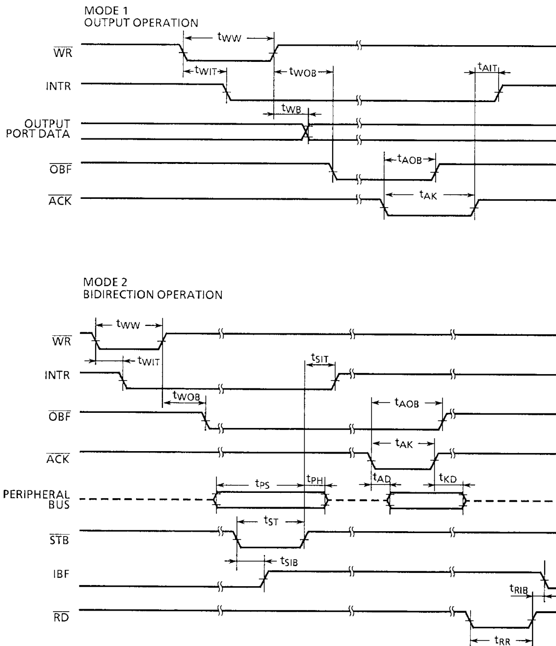
Figure 7.2 Timing diagram
