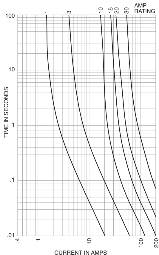
Time-Current Characteristic Curves—Total Clear
