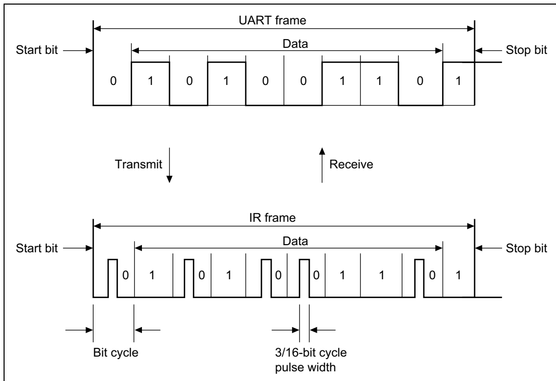
Figure 17.5 Transmit/Receive Operation
