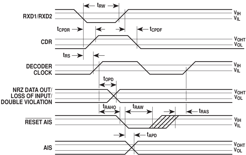
Figure 10 - Decoder timing parameters
