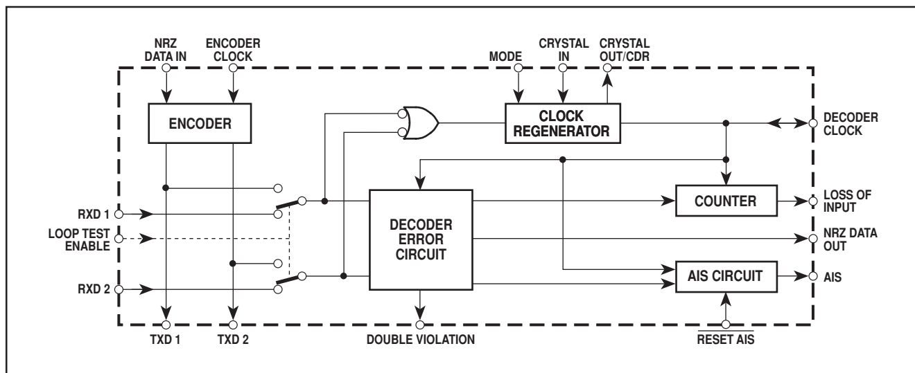
Figure 2 - Block diagram
