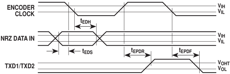
Figure 9 - Encoder timing parameters
