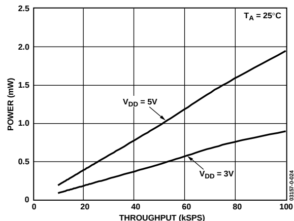
Figure 24. Power vs. Throughput Rate for SCLK = 10 MHz for V_{DD} = 3 V and 5 V
