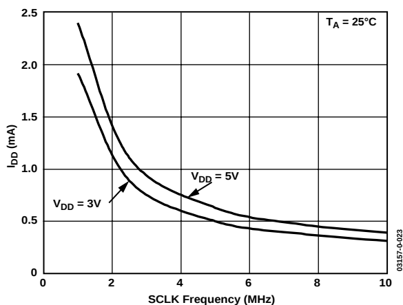
Figure 23. I_{DD} vs. SCLK Frequency for V_{DD} = 3 V and 5 V when Operating at 100 kSPS
