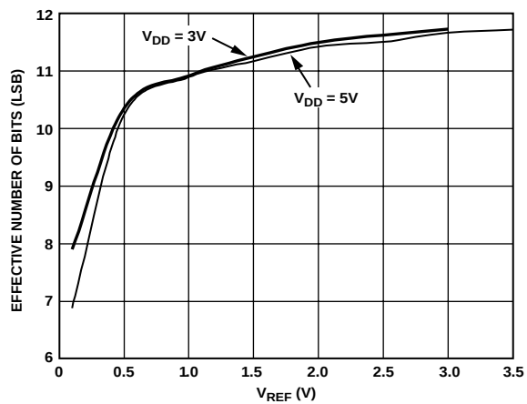
Figure 13. ENOB vs. V_{REF} for V_{DD} = 3\text{ V} and 5\text{ V}
