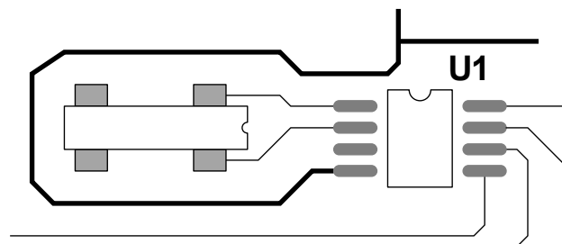
FIGURE 15. SUGGESTED LAYOUT FOR ISL12058 AND CRYSTAL
