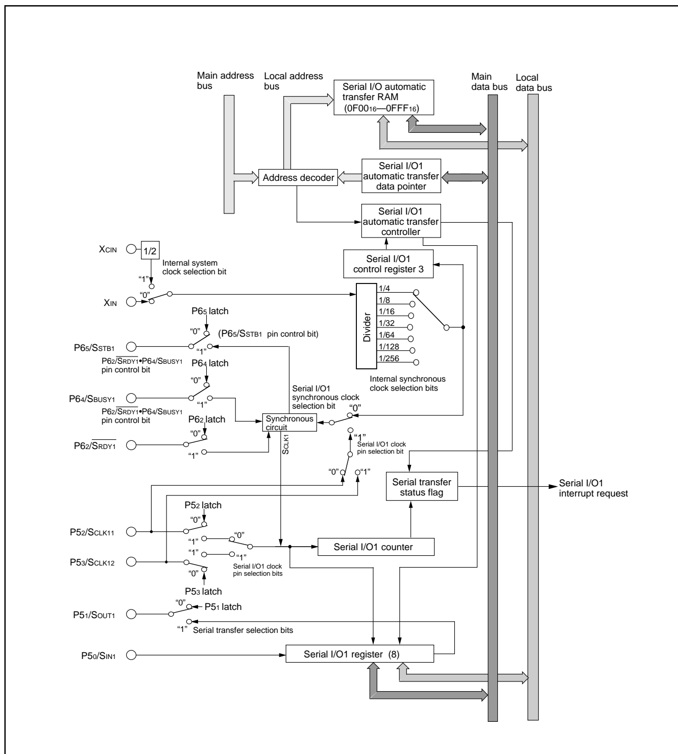
Fig. 19 Block Diagram of Serial I/O1
