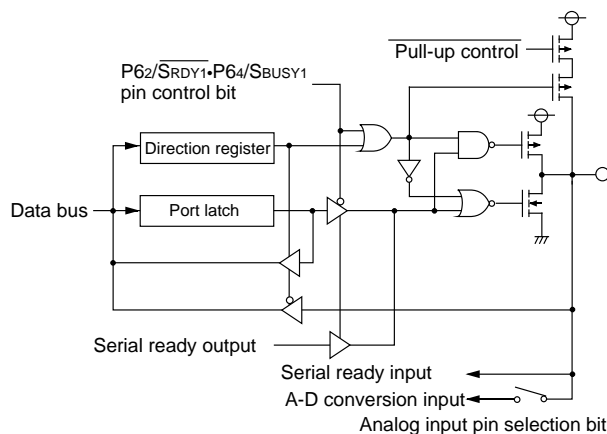
Fig. 10 Port Block Diagram (2)
