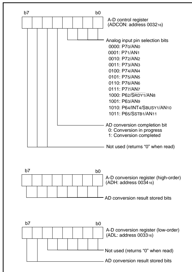
Fig. 51 Structure of A-D Control Register
