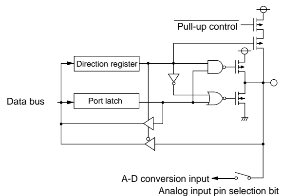
(14) Ports P63, P7
