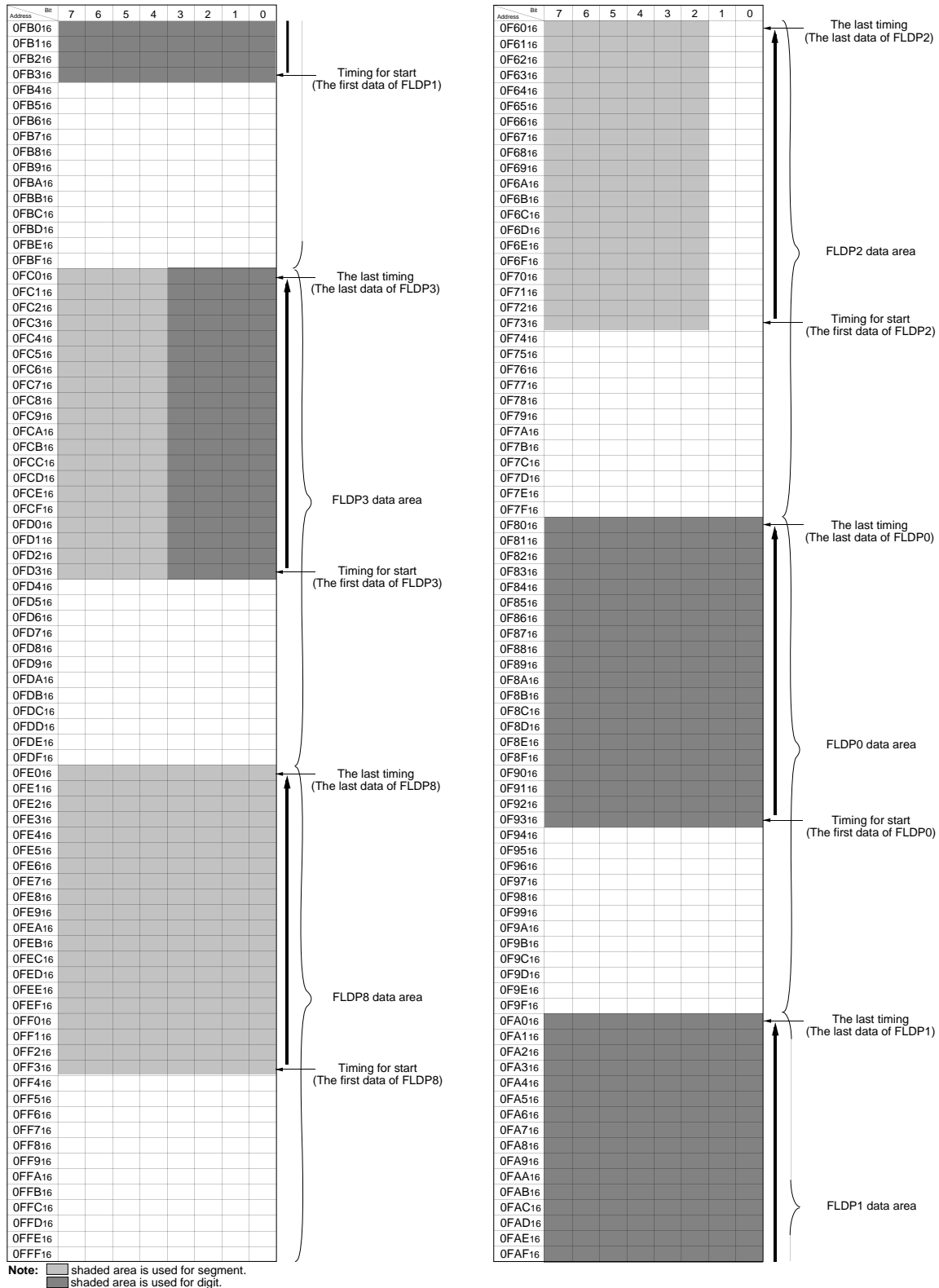
Fig. 45 Example of Using the FLD Automatic Display RAM in 32-timing Mode
