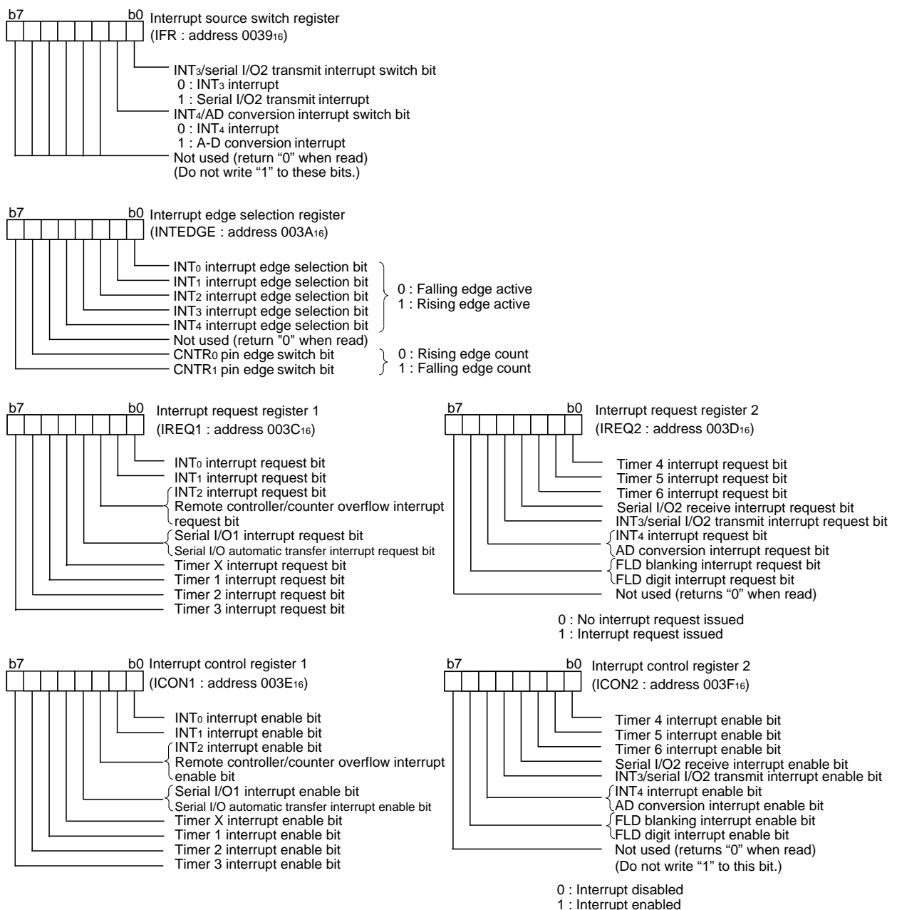
Fig. 13 Structure of Interrupt Related Registers
