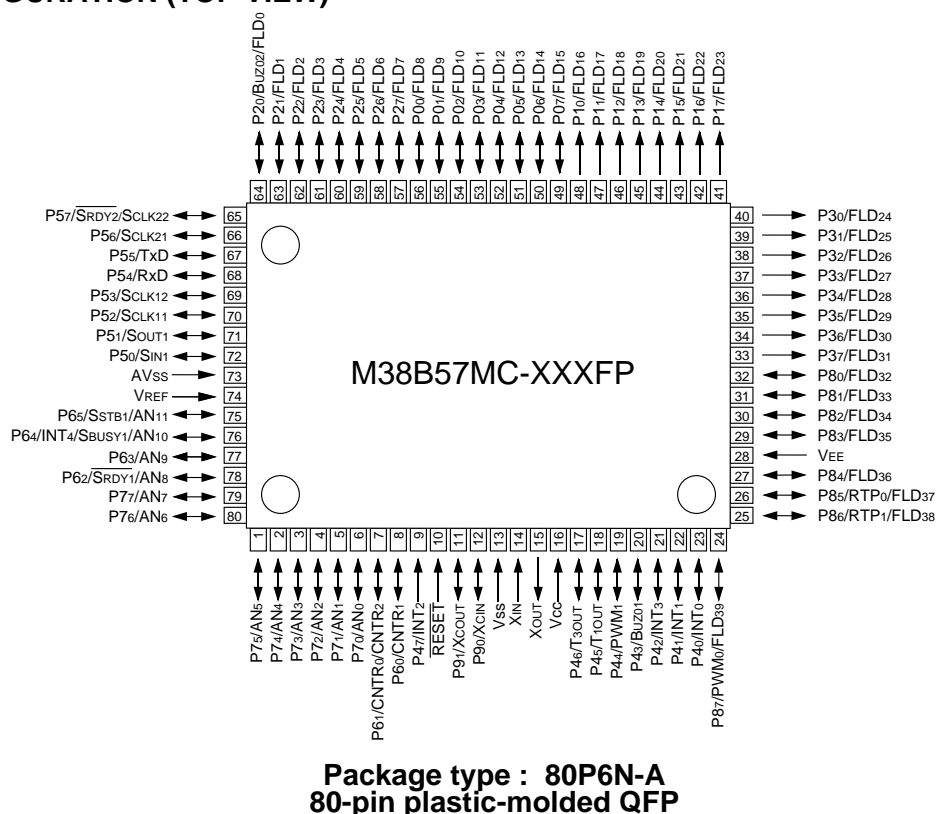
Fig. 1 Pin Configuration of M38B57MC-XXXXFP
