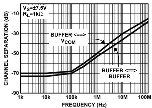
FIGURE 15. CHANNEL SEPARATION
