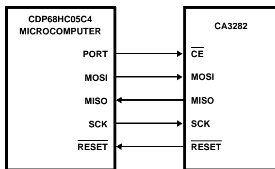
FIGURE 3. TYPICAL MICROCOMPUTER INTERFACE WITH THE CA3282
