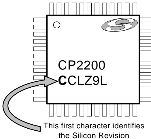
Figure 30. Device Package—TQFP 48
