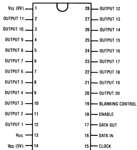
Figure 1. Dual-In-Line Package - Top View
