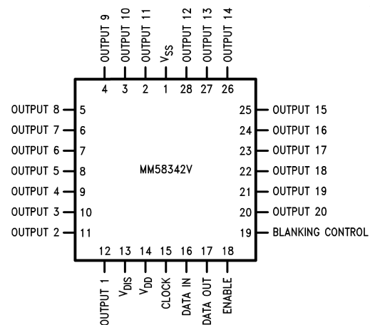
Figure 2. Plastic Chip Carrier - Top View Package PLCC (FN)
