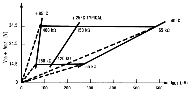
Figure 3. Output Impedance Off
